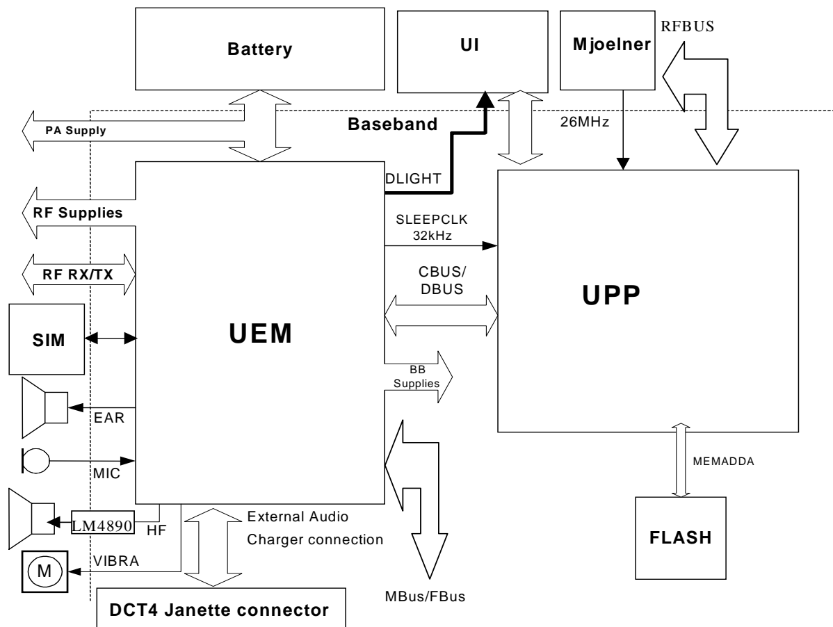
Figure 1: NPM-10 baseband block diagram
