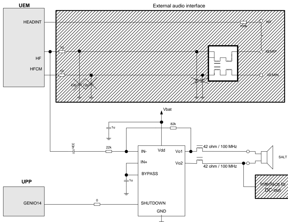
Figure 7: Ringer interface
