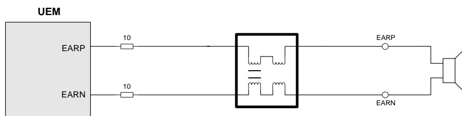
Figure 6: Speaker Interface
