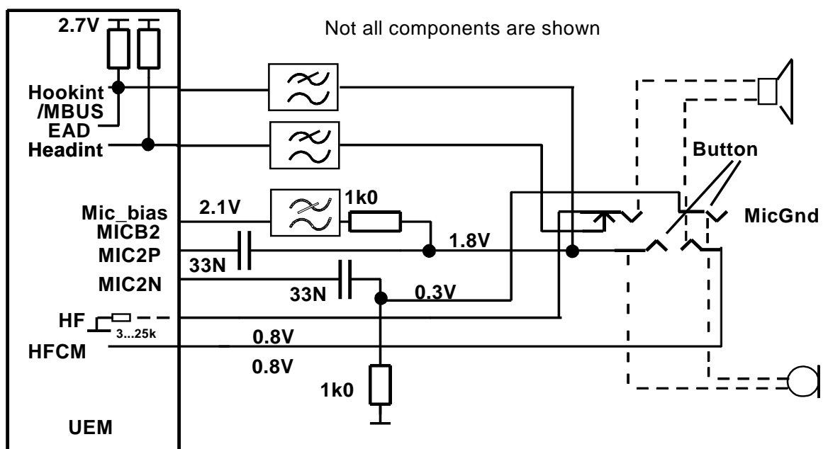
Figure 8: Headset interface
