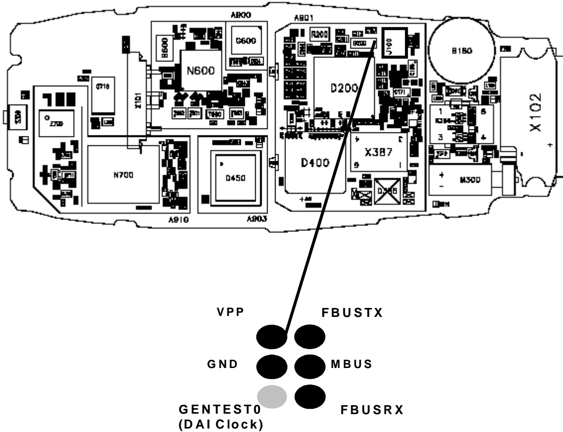
Figure 10: Production/Test/Customer Care interface
