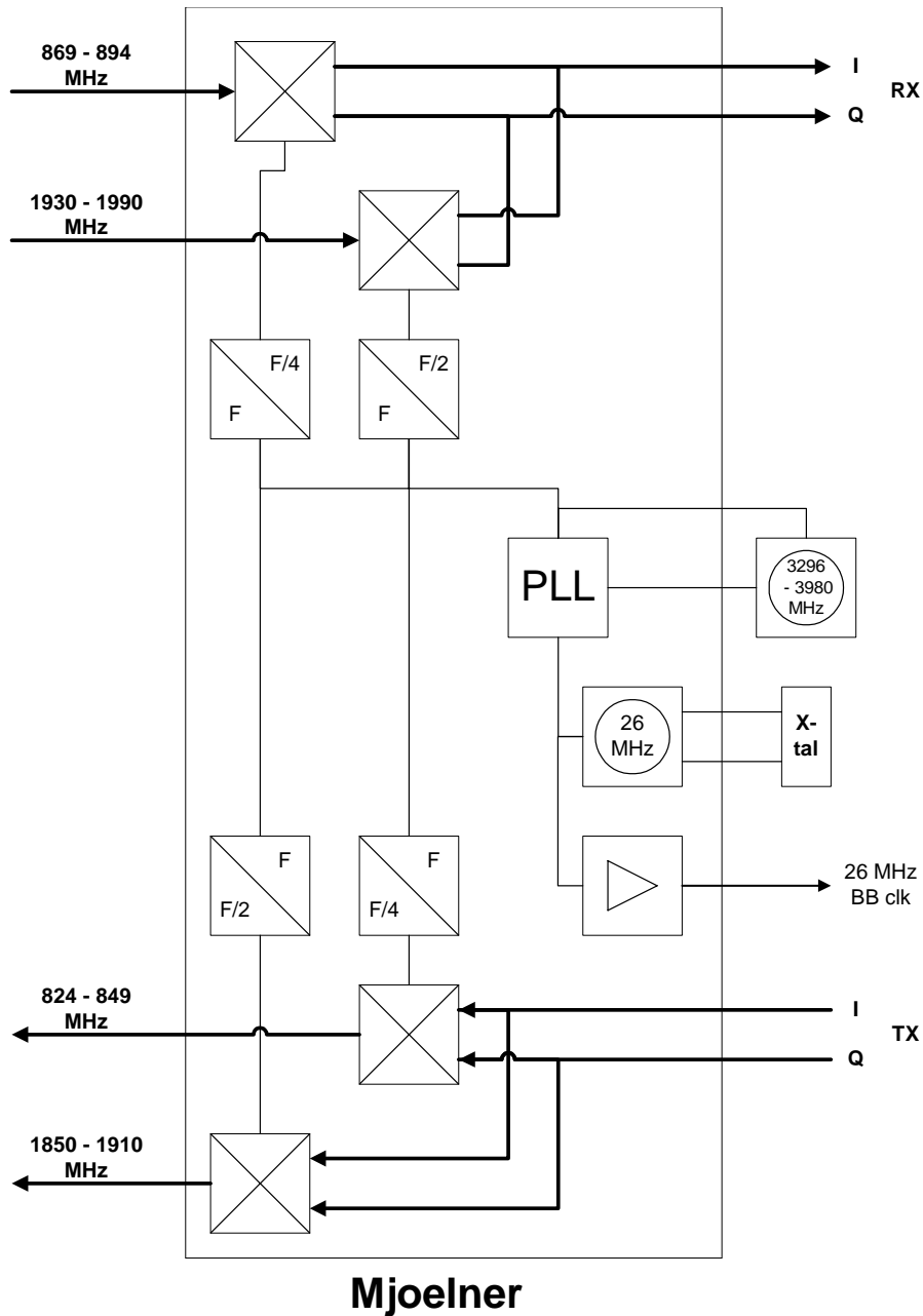
Figure 11: RF Frequency plan
