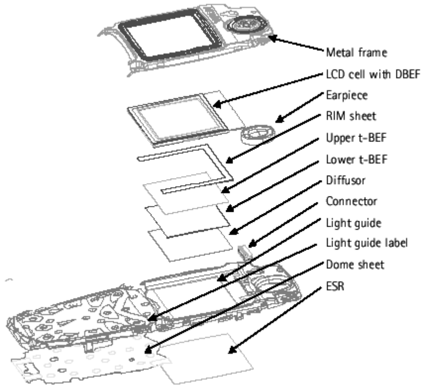
Figure 5: Overview of LCD module SIM Interface
