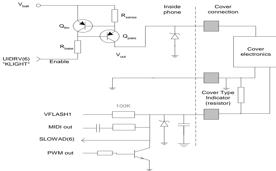
Figure 9: DC-OUT Interface
