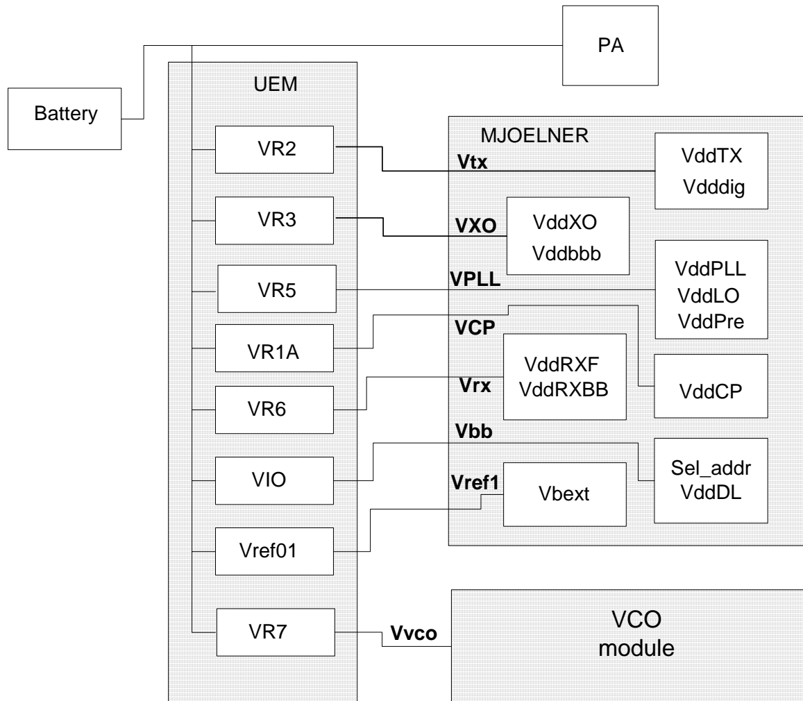
Figure 12: Power Distribution
