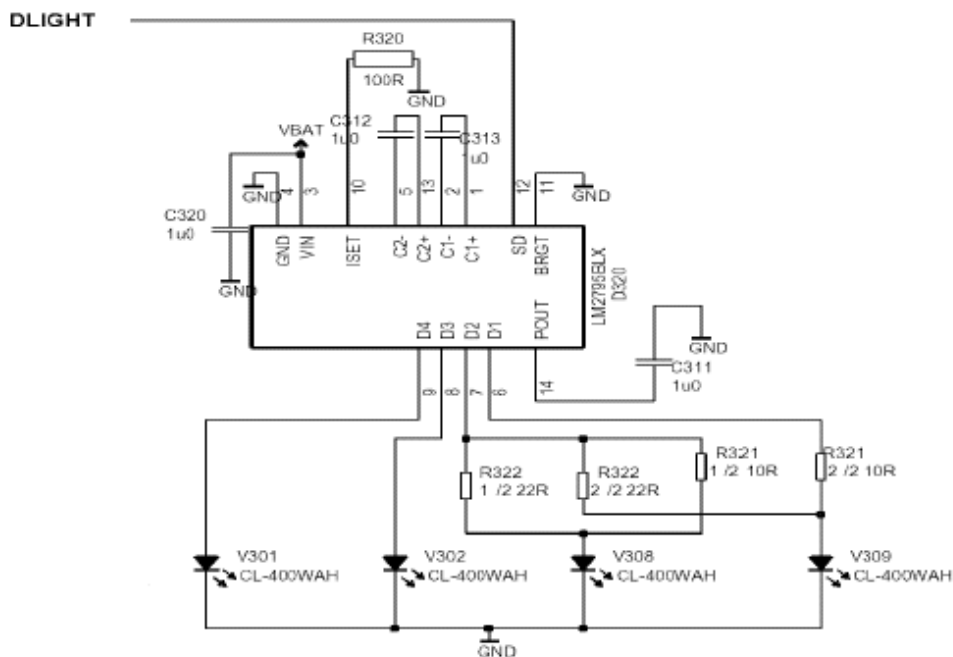
Figure 4: DLIGHT View
